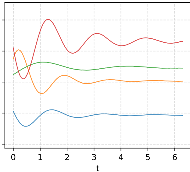
Flow matching
