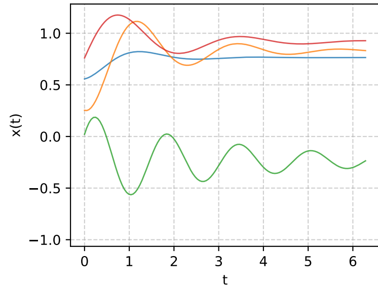
Original data
